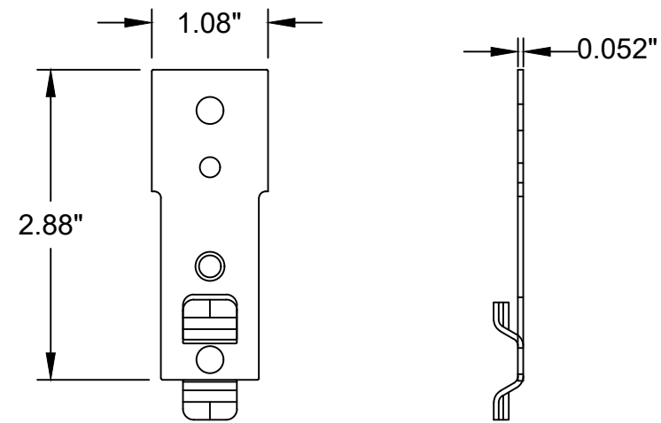
STRAP ANCHOR PART NO. 9858 GALVANIZED STEEL
