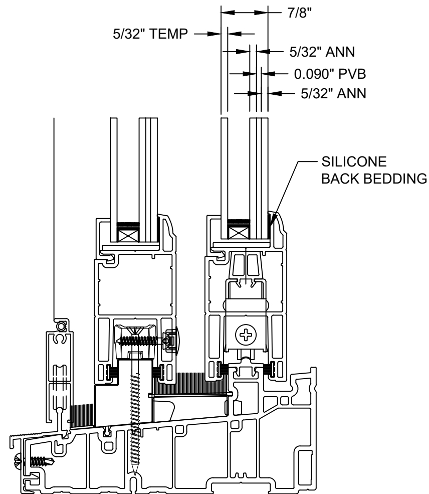
GLAZING DETAIL
